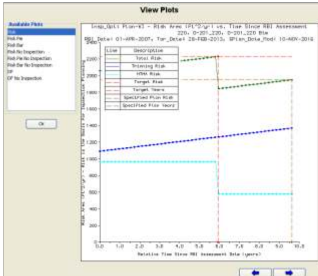
This plot shows the calculated damage progression over time, and “time stamped” date when the acceptable risk target will be reached. A recommended inspection plan is then generated based on the percentage of total risk by each individual damage mechanism.
